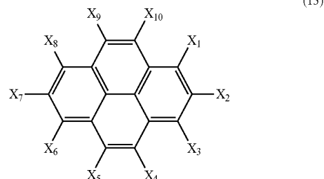
[Chemical Formula 13]
