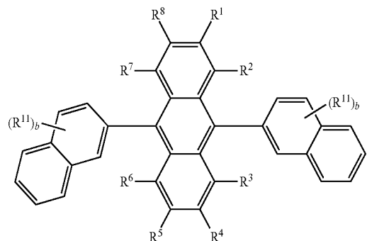
[Chemical Formula 4]
