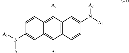
[Chemical Formula 11]
