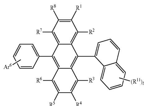
[Chemical Formula 5]
