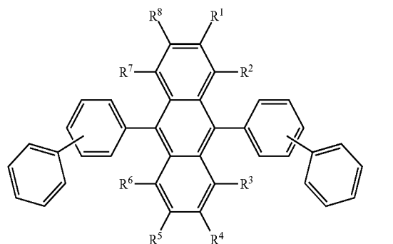
[Chemical Formula 9]
