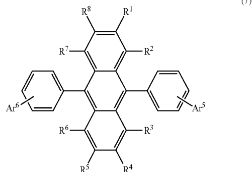
[Chemical Formula 7]
