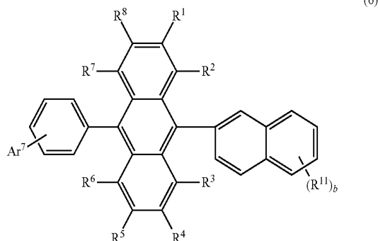
[Chemical Formula 6]
