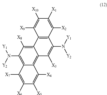
[Chemical Formula 12]
