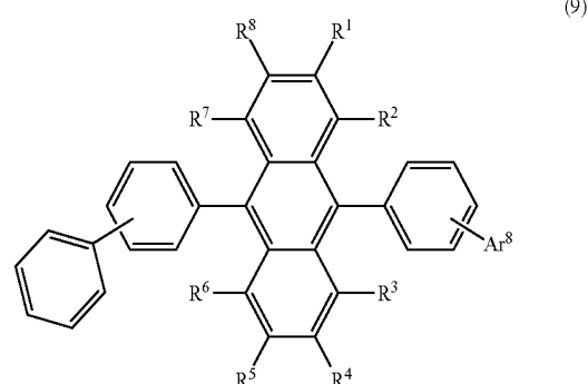
[Chemical Formula 9]
